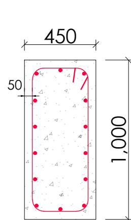
SF2 Footing
