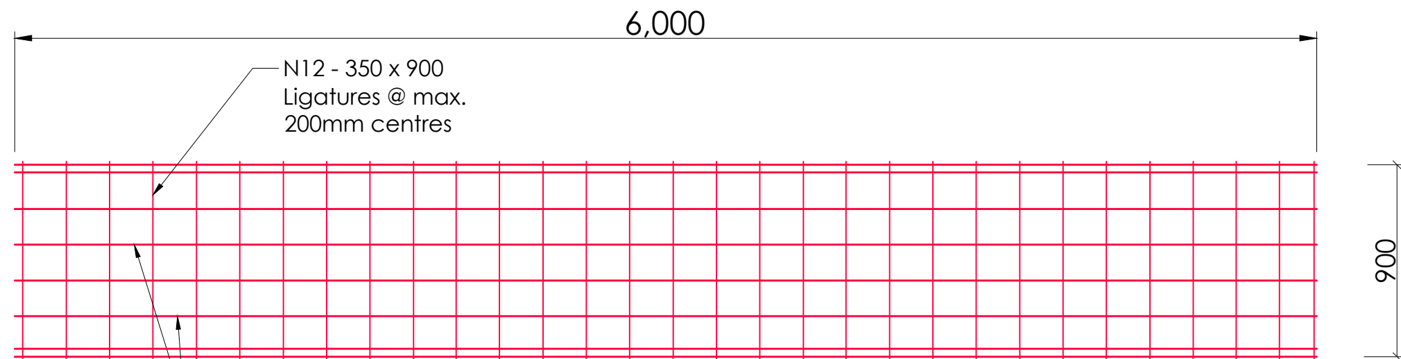
Side View
