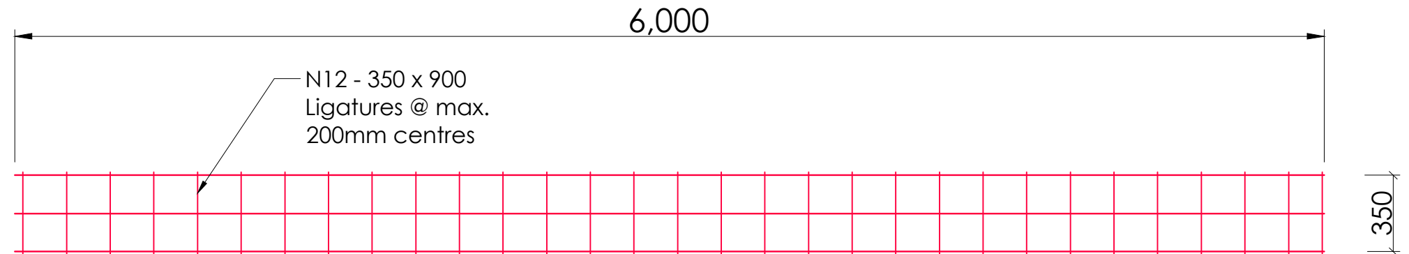
Top View
