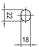
DETAIL SLOTTED HOLES 1:5
