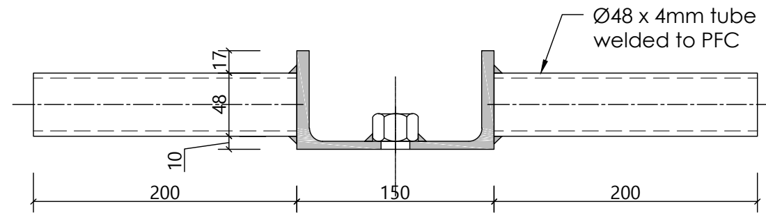
Section
