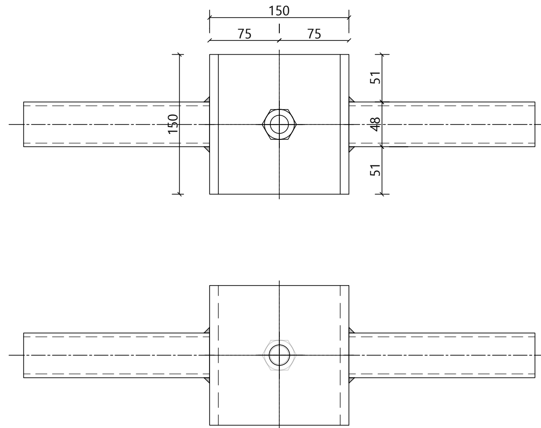
Column Bracing in Y-Y plane
