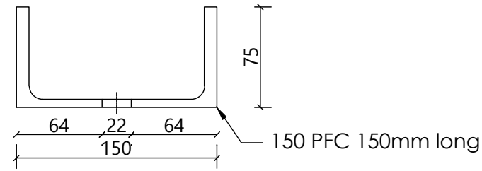
Section
