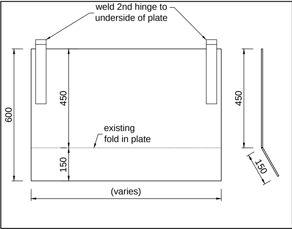
Weld 2nd hinge to Plate (Viewed from Underside of Plate)
