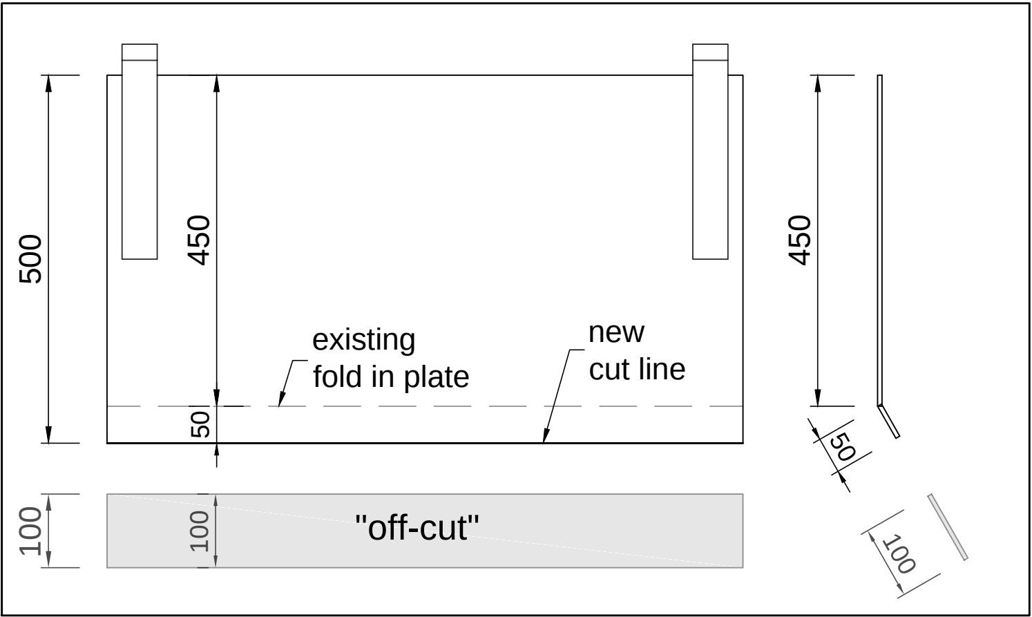
Cut 100mm wide strip full length of plate
