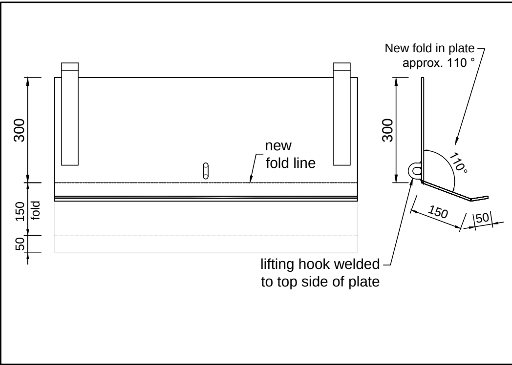
Fold Plate & Weld Lifting Hook
