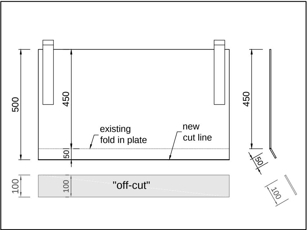
Cut 100mm wide strip full length of plate
