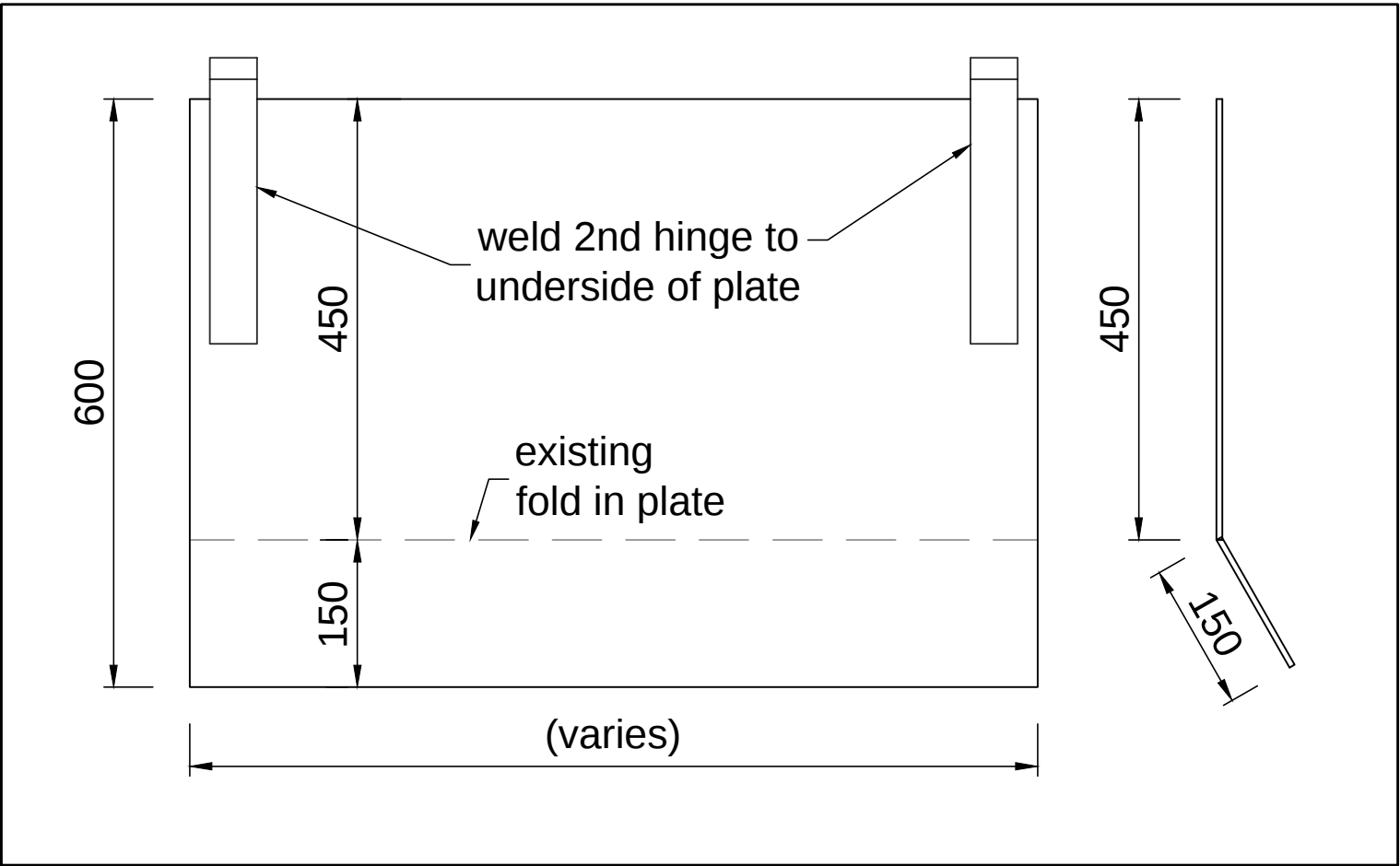
Weld 2nd hinge to Plate (Viewed from Underside of Plate)
